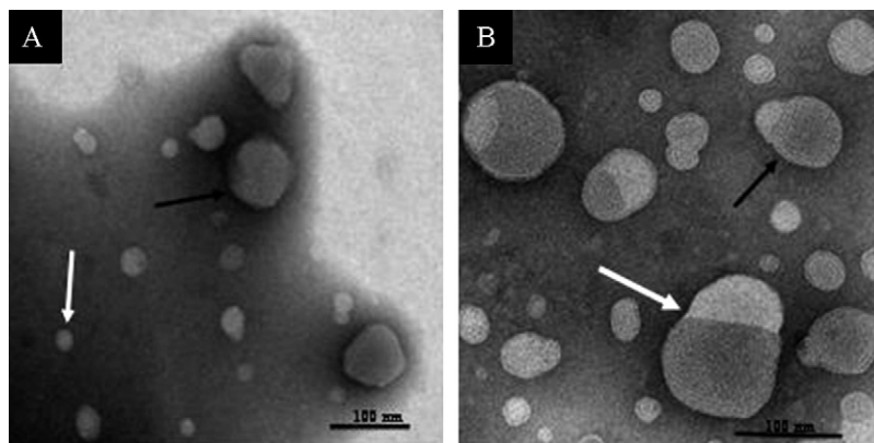
Fig. 3. Nanoscale multicompartiment liposome (MCL) consists of small unilamellar vesicles (SUV) (white arrow) separated from multilamellar vesicles (MLV) (black arrow) by interface, prepared by extrusion of micrometer-sized MCL. Transmission electron microscopy image (TEM) of 1% PTA stained LUV:SUV mixing system (A) and MCL system (B).
